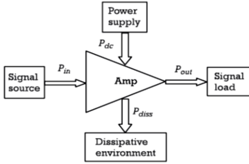
Figure 1. Power inputs and output on PA [2].
