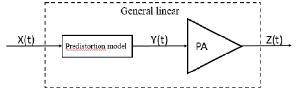
Figure 2. Predistortion technique [4].
